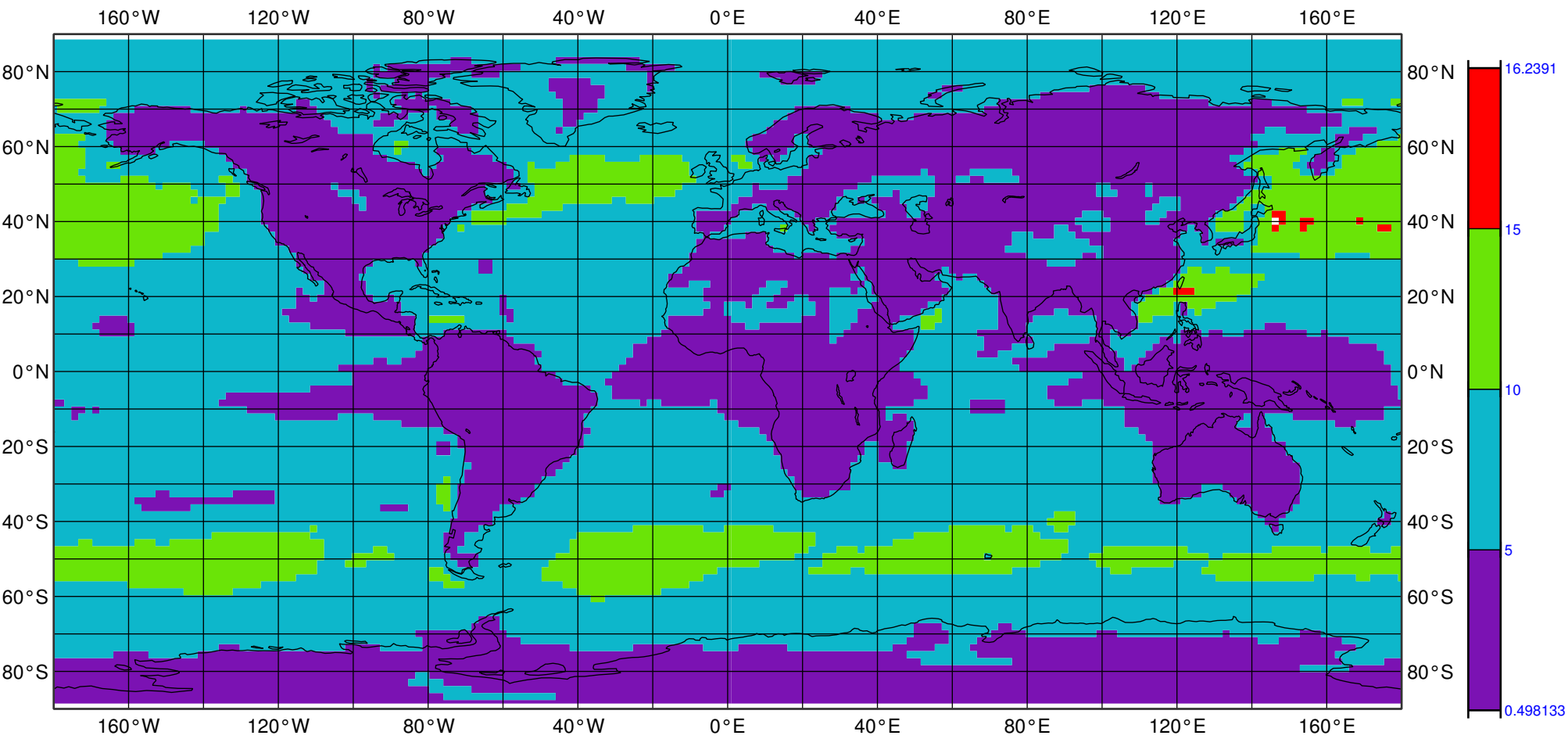
wind10 [m/s] 1866-02-15 02:52:00
