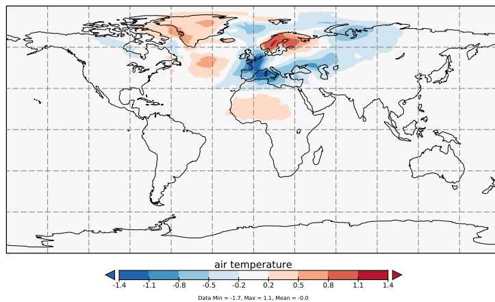
1709 Jan: cycle2 - cycle1
