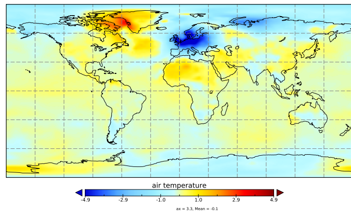
1709 Jan: cycle2 - cycle1
