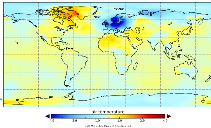
1709 Jan: cycle2 - model.clim
